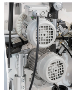
Buffing station
